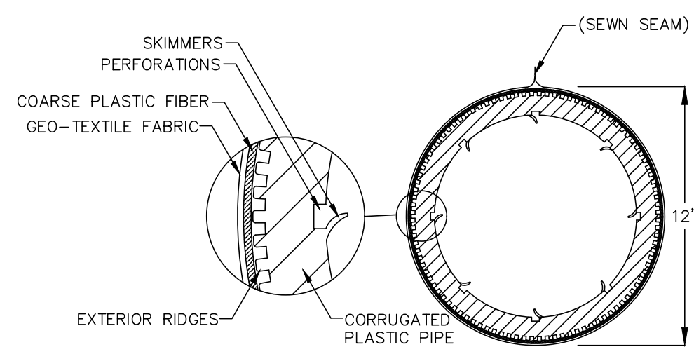
ENVIRO-SEPTIC LEACHING SYSTEM
