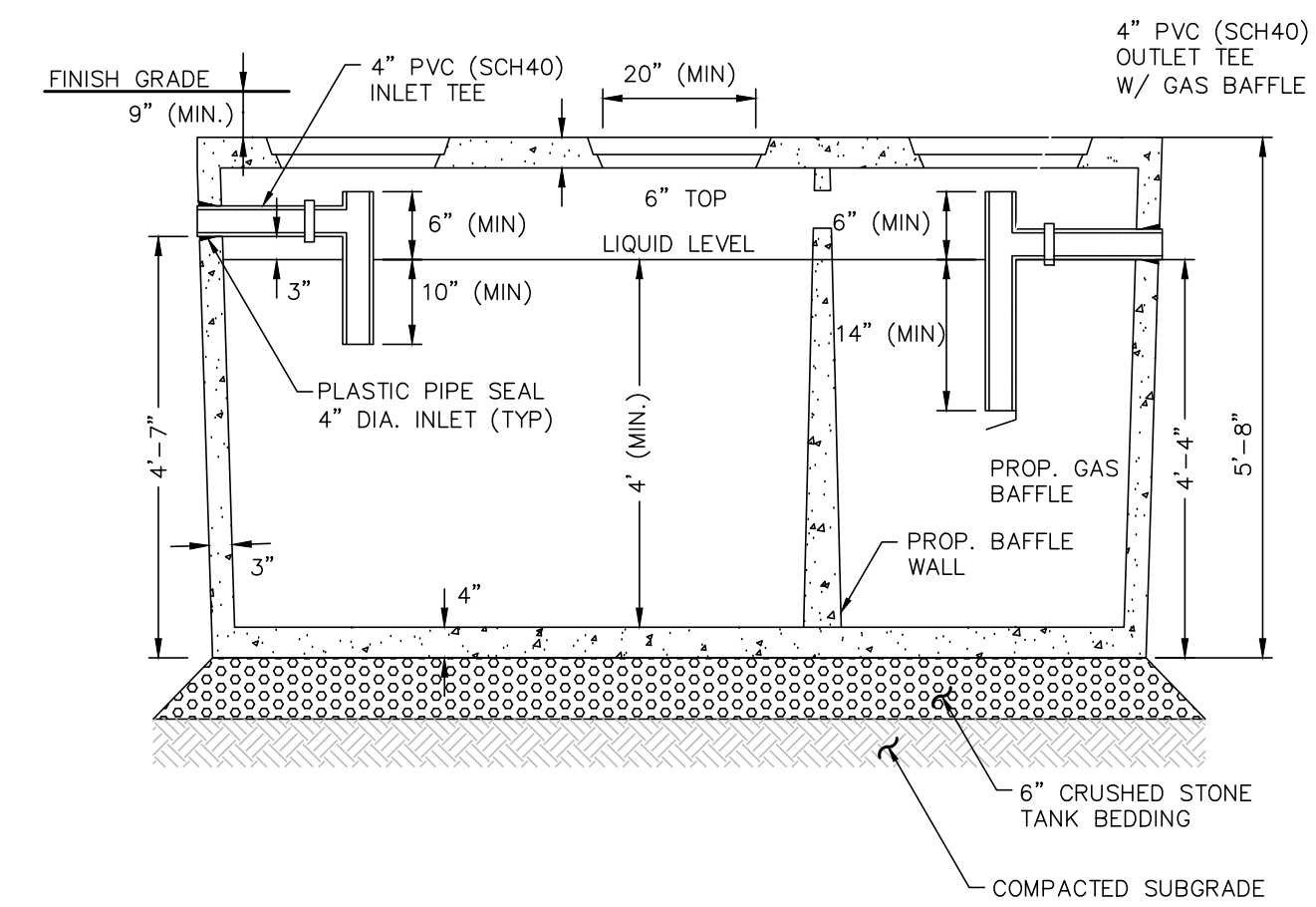
SEPTIC TANK SECTION VIEW
