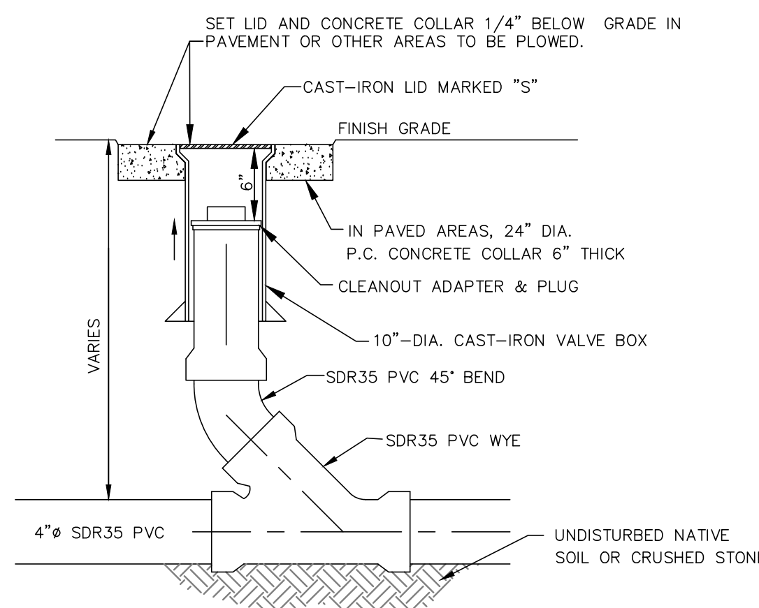
TYPICAL SEWER CLEANOUT
