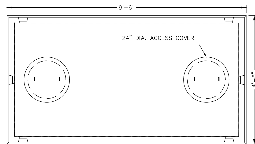
PUMP CHAMBER PLAN VIEW
