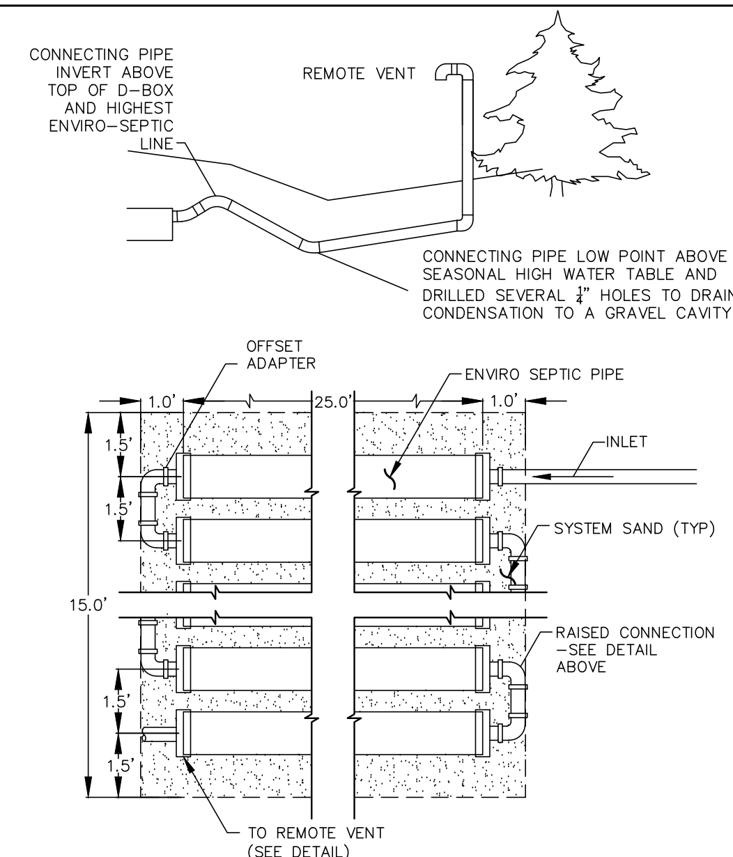
SYSTEM CONFIGURATION AND VENT DETAIL
