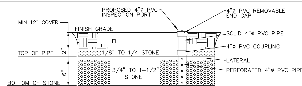
INSPECTION PORT DETAIL
