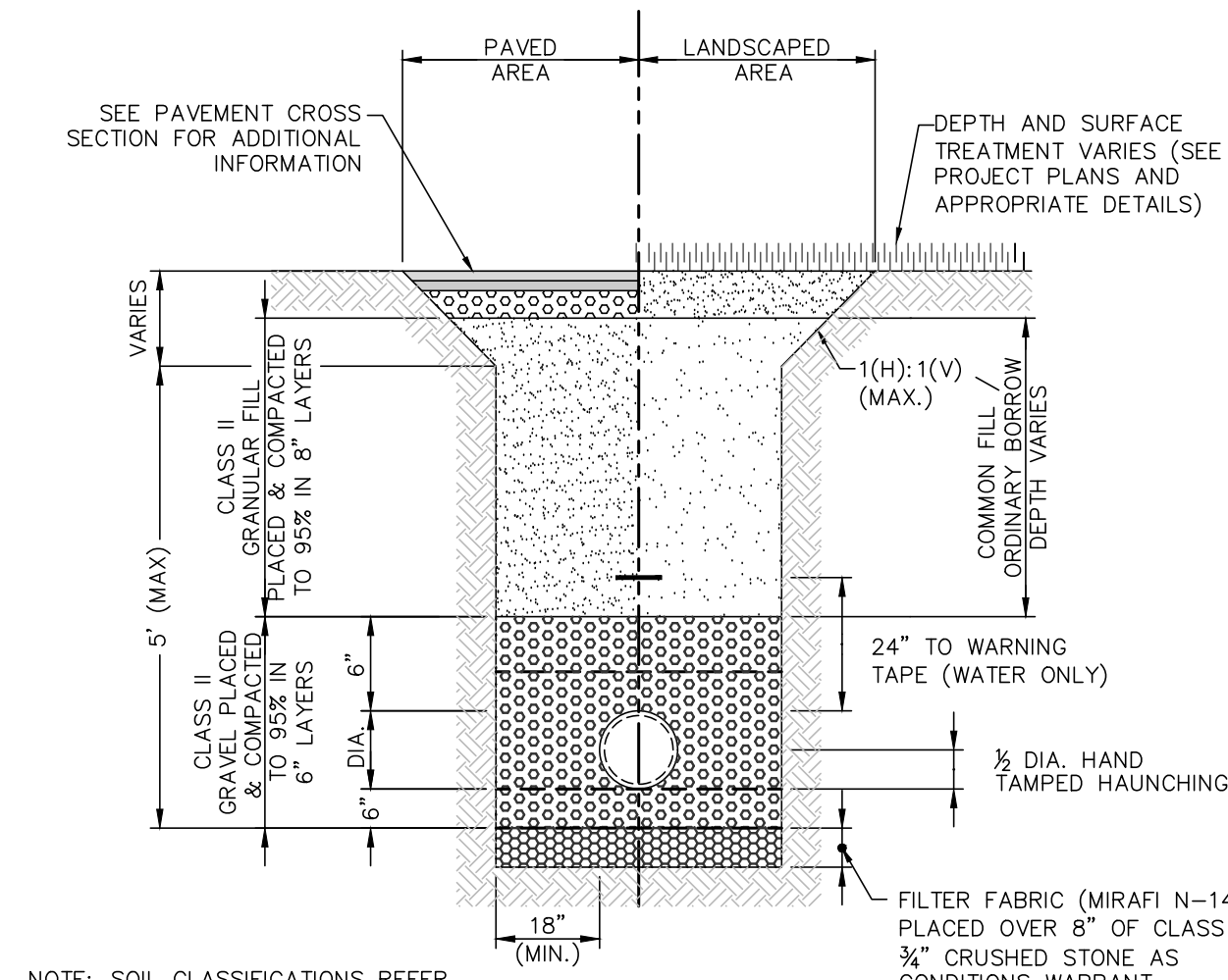
TYPICAL UTILITY TRENCH DETAIL
