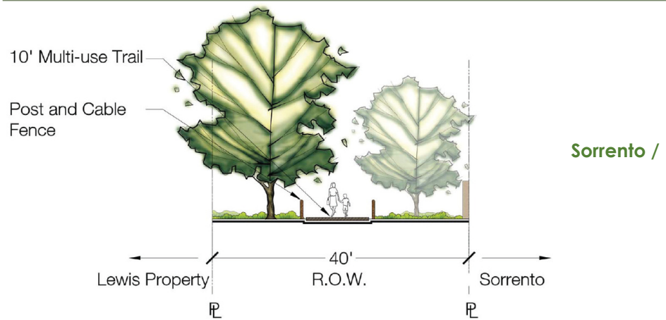
Figure 7-16: Section D1-D2: Village 7 Trail Corridor
